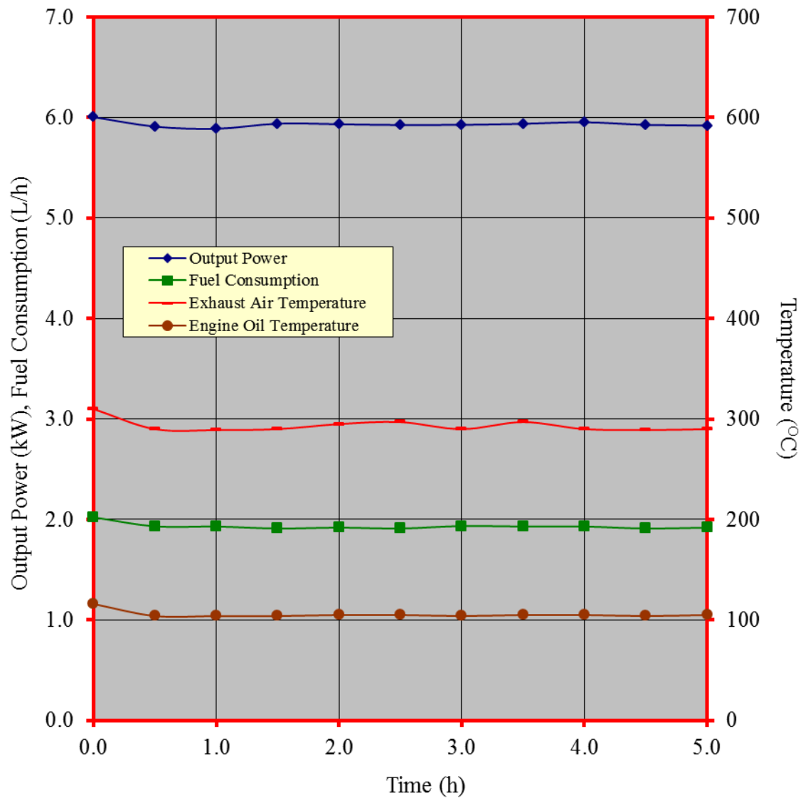
Figure 4. Performance characteristic curves during the continuous running test of the TOPTEK BT186 diesel engine
