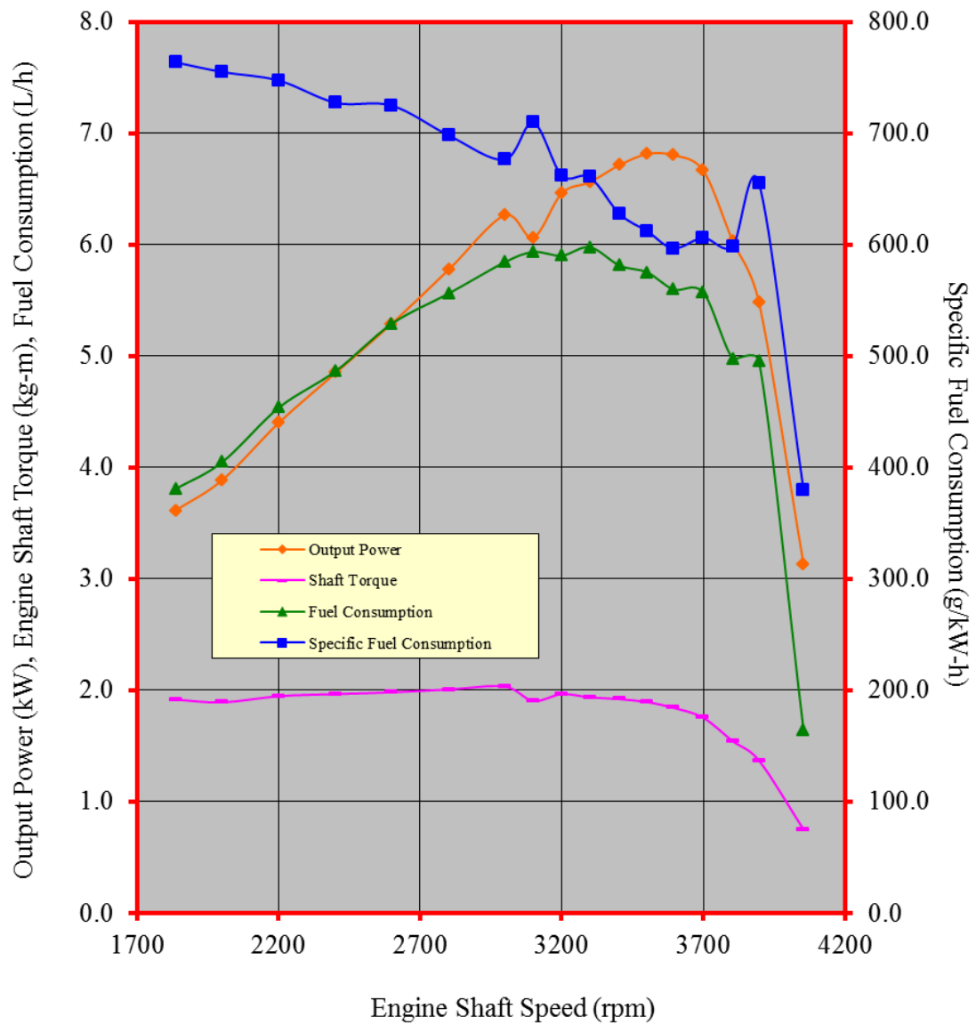
Figure 3. Performance characteristic curves of the TOPTEK BT186 diesel engine
